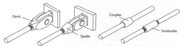
TIE RODS AND FITTINGS
