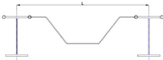
ESC - H/1 COMBINATION PILES
