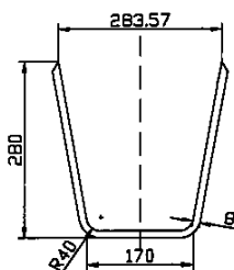
U-BEAM
