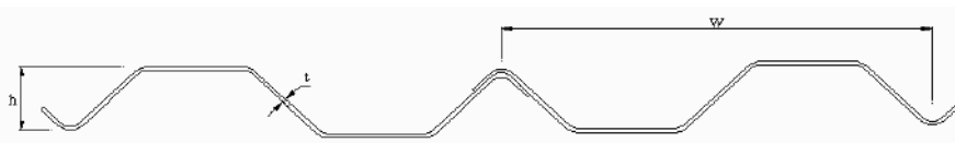
ESC - TRENCH SHEET PILE COLD FORMED
