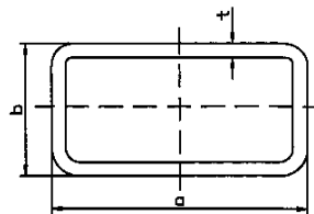
RECTANGLE TUBE
