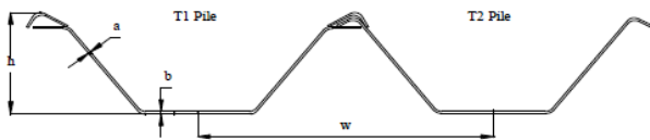
ESC - B WIDE PROFILE SHEET PILE COLD FORMED
