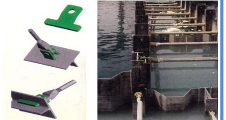
TIE RODS AND FITTINGS
