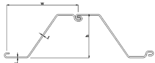
ESC - CRZ SHEET PILE COLD ROLLED
