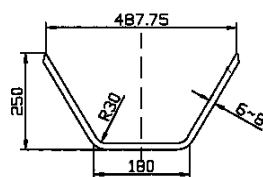
U-BEAM
